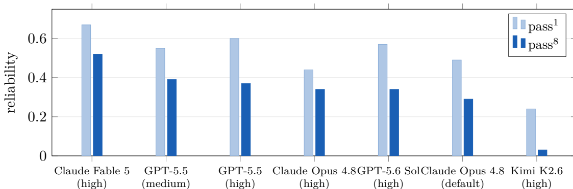
Figure 1: The reliability gap. \text{pass}^1 (the chance one run succeeds; mean single-run success rate) versus \text{pass}^8 (the chance all 8 succeed) for each model configuration.
