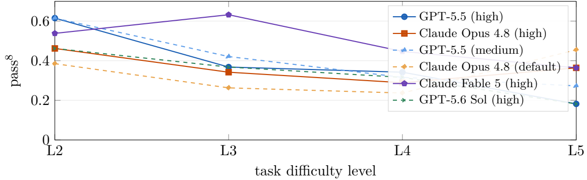
Figure 3: \text{pass}^8 by difficulty. The L5 inversion (Claude overtaking GPT-5.5) reflects task mix, not a clean difficulty gradient.
