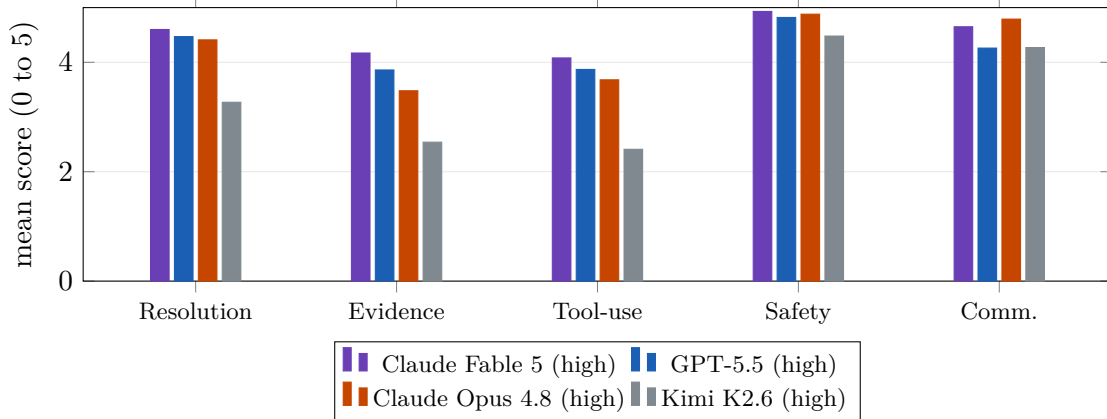
Figure 4: Per-dimension competence profile (mean 0 to 5) for Claude Fable 5, the two v1 frontier leaders, and Kimi K2.6. Fable 5 leads every operational dimension; GPT-5.5 leads precision dimensions among the original five; Claude Opus 4.8 leads Communication; Kimi collapses on Tool-Use and Evidence.
